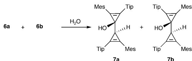
Scheme 4. Spontaneous addition of water to triafulvalenes 6a and 6b .
